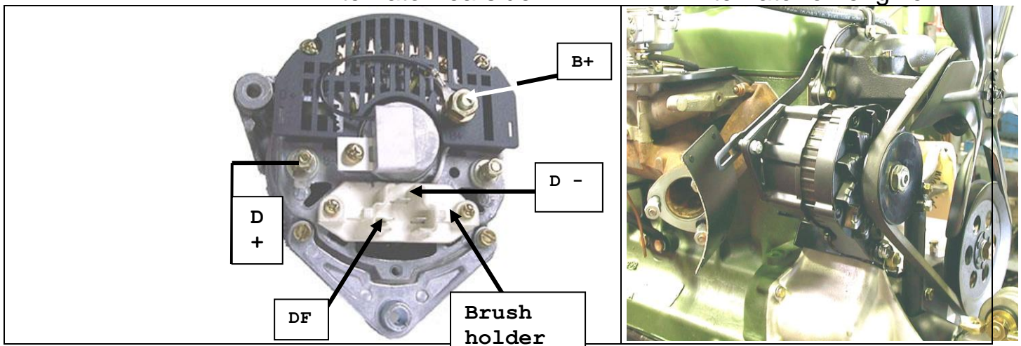
Alternator rearside.
