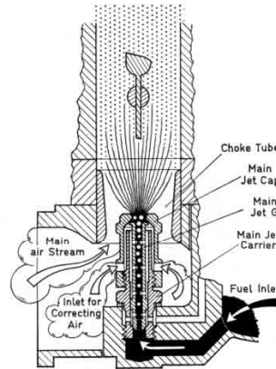
Fig. 20 Main jet circuit of a updraught carburetor
