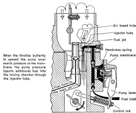
Fig. 33 Accelerator pump of the 28 PCI carburetor
