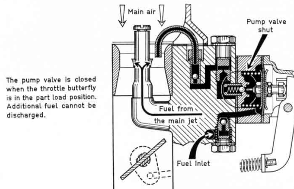
Fig. 34 "Rich" pump with ball valve (pump 73)
