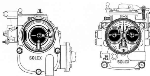
Fig. 3 Types of carburetors
