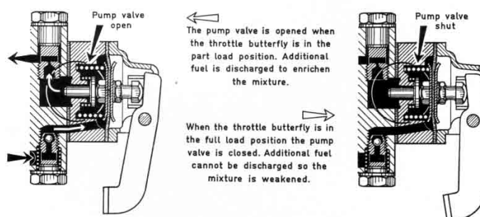
Fig. 36 "Weak" pump with disc valve (pump 84)
