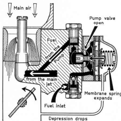
Fig. 30 Depression operated accelerator pump
