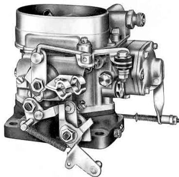
Type 32 PAITA (Downdraught Compound Carburetor)
