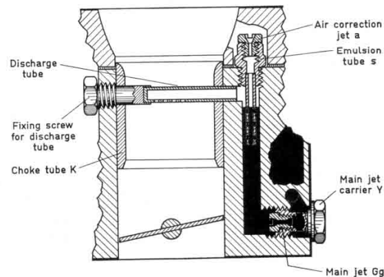
Fig. 28 Jet assembly of the 40 PII carburetor
