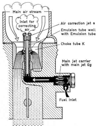
Fig. 19 Main jet circuit of a downdraught carburetor
