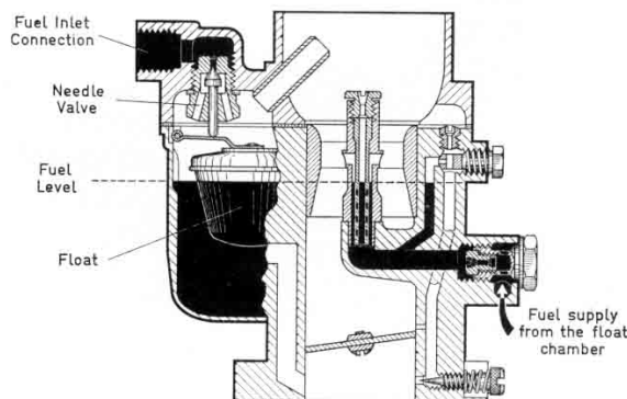
Fig. 6 The Float System
