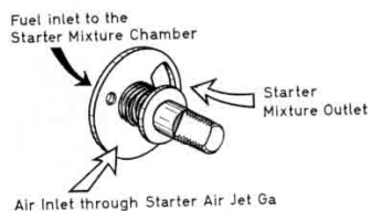
Fig. 8 Disc Valve of a simple Starter
