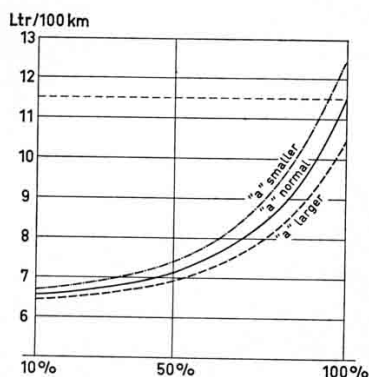
Fig. 22 Diagram of the affect of the air correction jet a
