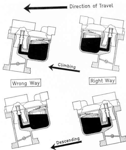
Fig. 4 Position of the Float Chamber
