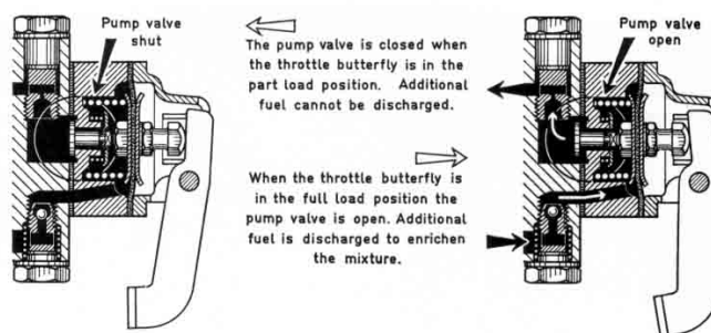
Fig. 35 "Rich" pump with disc valve (pump 83)
