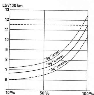
Fig. 21 Diagram of the affect of the main jet Gg
