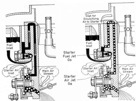
Fig. 7 Operation of the Starter Disc Valve
