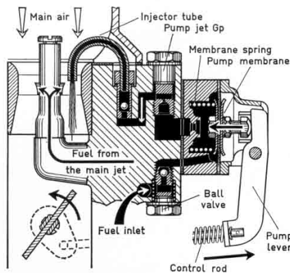
Fig. 29 Mechanically operated accelerator pump
