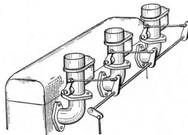
Fig. 5 Control layout for multiple carburetors
